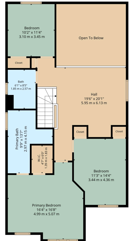
2nd Floor
